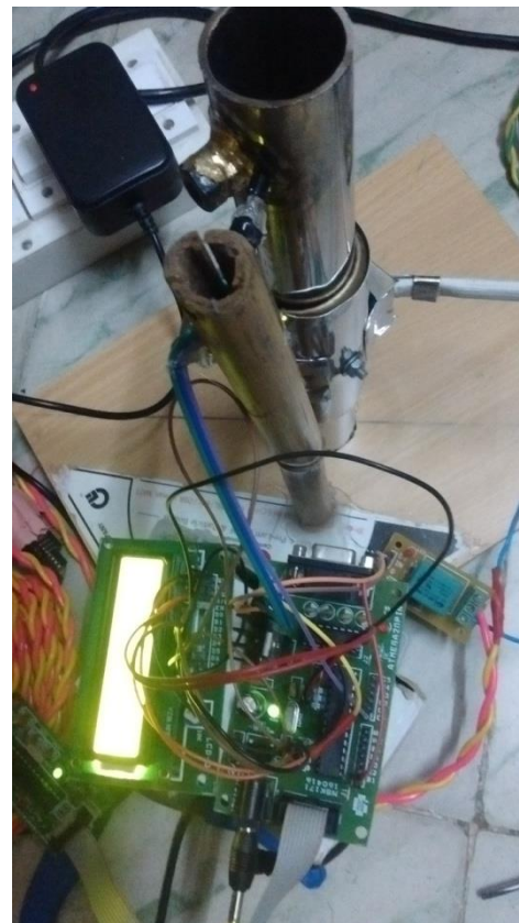
Temperature Multi Threshold Cut Off (For A Cement Factory Unit)
