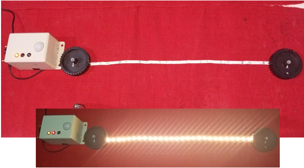
Cot Attached Magical Night Light (Timer Adjustable)
